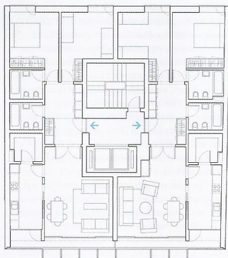
Planta 2. 2 Floor.
